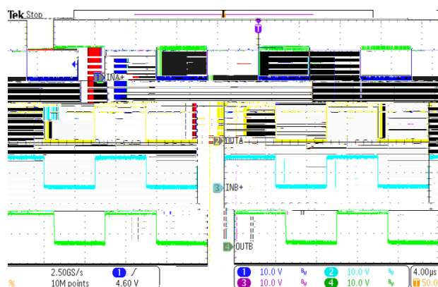
Application Waveform
